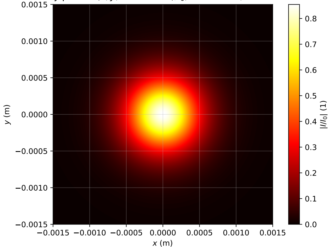
Intensity profile I(x, y, z = 2.946m)/I_0 , P_{in}=0.7P_{cr} , artificial time
